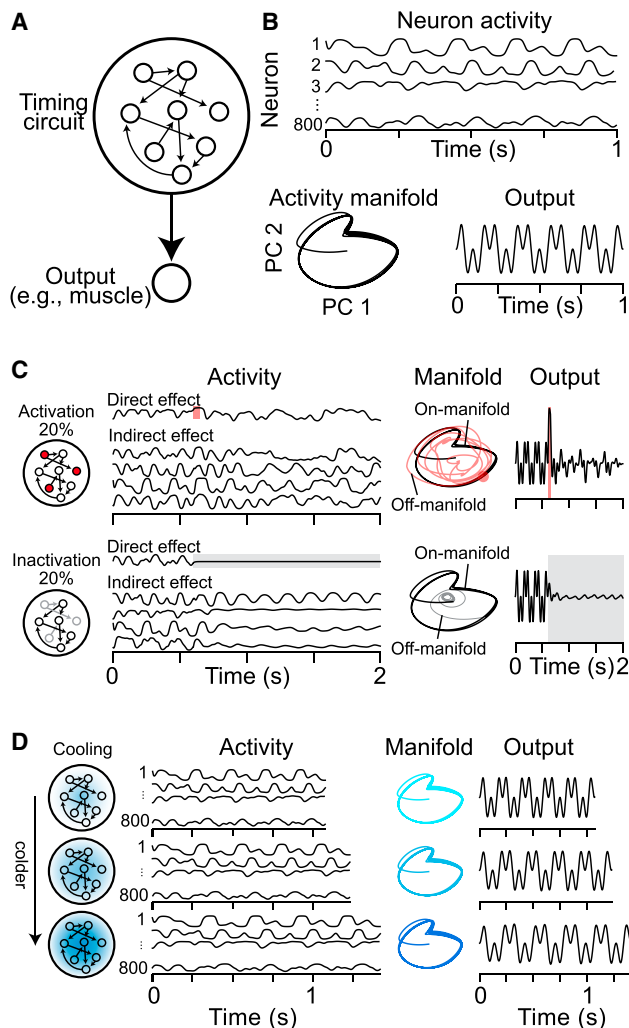
Figure 5. Manipulations in a recurrent neural network (A) Schematic of our timing circuit model which consists of 800 rate-based neurons forming an all-to-all recurrent neural network with random synaptic weights drawn from a normal distribution scaled by a factor g/\sqrt{N} , with g set to 1.5 (Sussillo and Abbott, 2009). Additionally, all neurons synapse onto a single output unit. Recurrent and output weights are updated using the FORCE algorithm (Sussillo and Abbott, 2009) to learn a desired output pattern (Laje and Buonomano, 2013). (B) Activity of four example neurons after learning (top). Network activity structure visualized using the first two principal components (PCs; bottom left) and a learned output signal (bottom right). (C) Simulated large-scale manipulations and their effects on neuronal activity (left), network dynamics (center), and output (right). Shown here are responses to activation (top row, shaded red area) and persistent (bottom row, shaded gray area) inactivation of 20% of neurons within the simulated network. (D) Simulated cooling manipulation through three monotonically increasing levels of focal cooling. Mild cooling was modeled by augmenting network dynamics by a factor Q : \tau \frac{d\vec{x}}{dt} = -\vec{x} \cdot Q + W_{rec} \cdot \tanh(\vec{x} \cdot Q) , \vec{r} = \tanh(\vec{x}) . Here, \tau = 10\text{ms} , W_{rec} is the recurrent weight matrix, and \vec{x} and \vec{r} are vectors of length N describing the internal dynamics and firing rates of each neuron. Temperature dependence of Q was modeled using Q_{10} = 2 .
